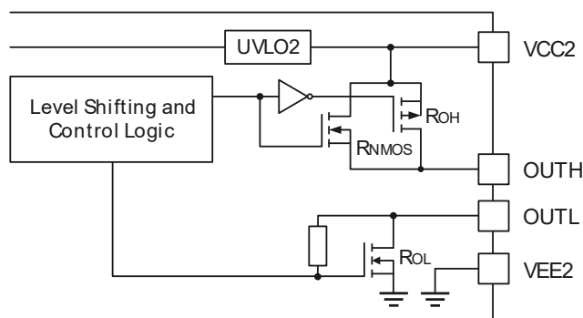
Figure 29. Output Stage
