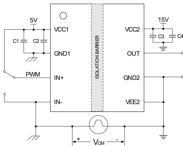
Figure 5. CMTI Test Circuit for BTD5350Ex
