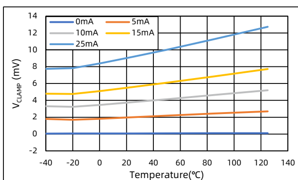
Figure 17. V_{CLAMP} vs. Temperature
