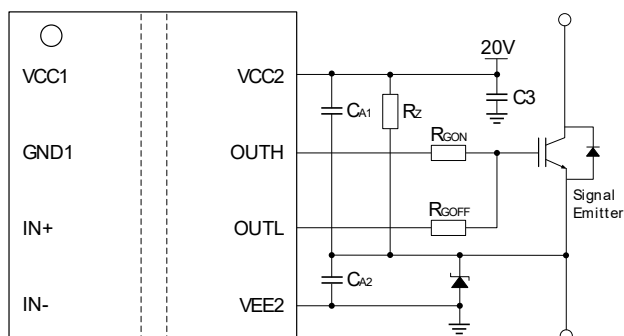
Figure 35. Voltage Regulator Design
