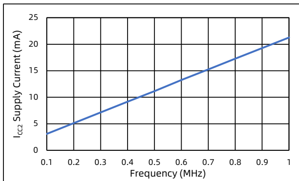
Figure 15. I_{CC2} power supply current vs. Input frequency
