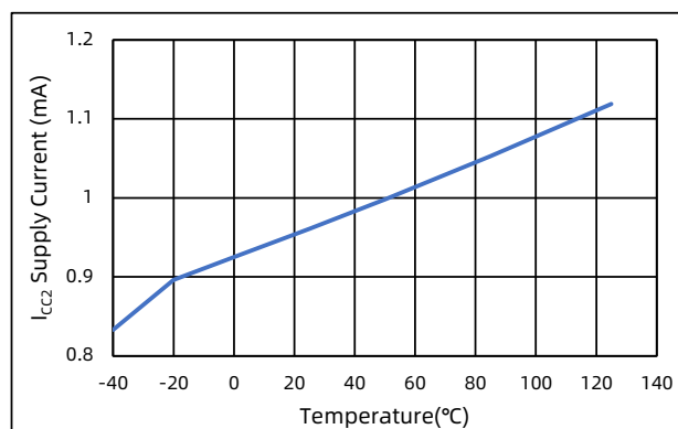
Figure 13. I_{CC2} power supply current vs. Temperature (IN+=L, IN-=H)
