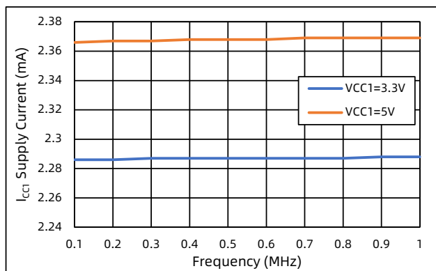
Figure 12. I_{CC1} power supply current vs. Input frequency
